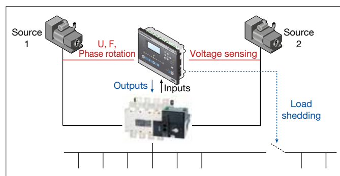
Switch-based (PC)
