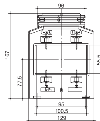
TBA 100 from 600 to 2500 A (1) T2BA 100 from 1200 to 3000 A
