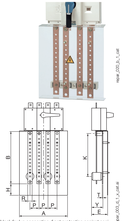
Distribution block for lug connection, front protection against accidental contact (switching device not included).
