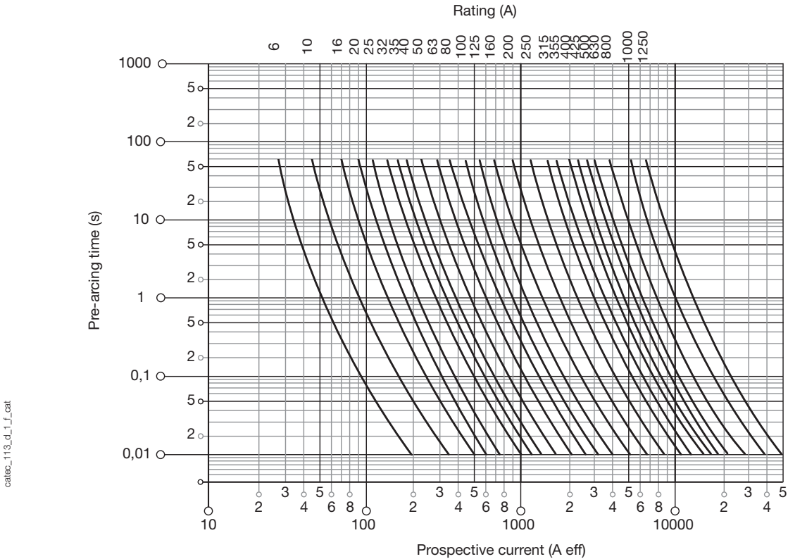
Time/current operation characteristics
