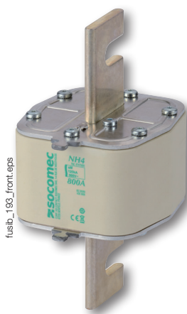
aM type fuse, NH4 315 to 1250 A
