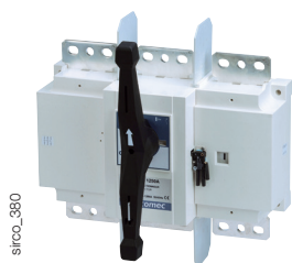
SIRCO 3 x 1250 A with early pre-break AC
