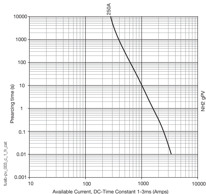
gPV cylindrical fuses 14x51
