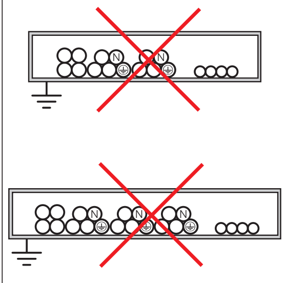
Incorrect installation
