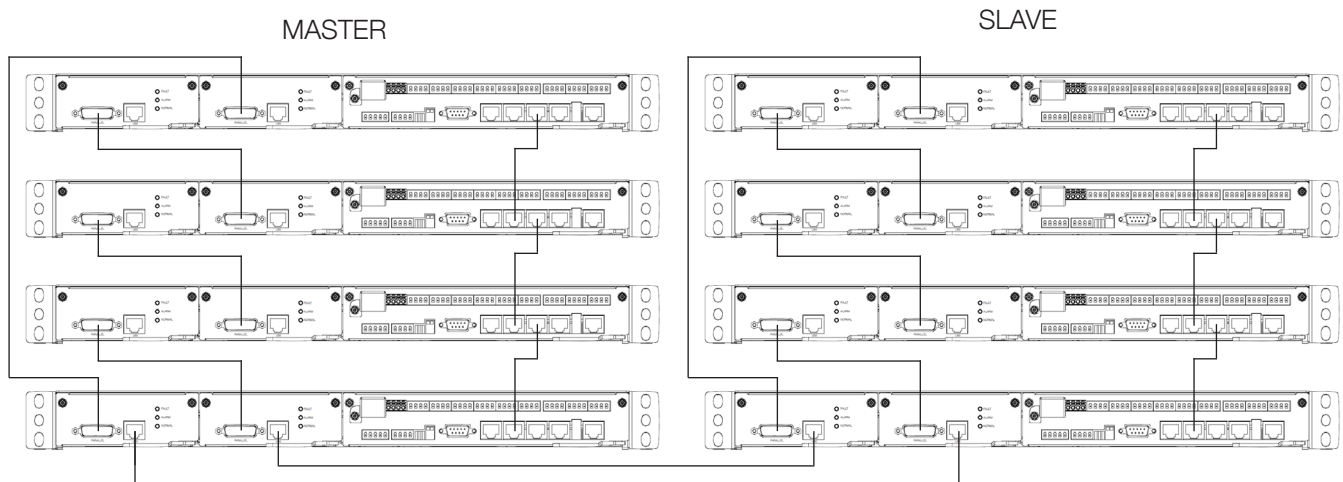
PARALLEL UPS SYSTEM LBS CONNECTED TO STS
