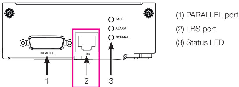
SINGLE UPS SYSTEM LBS
