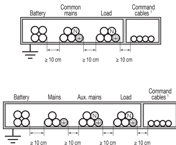
Authorised installation
