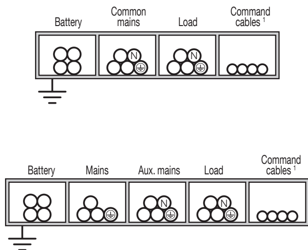
Correct installation
